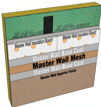
Aggre-flex Drainage EIFS with Drainage Mat
