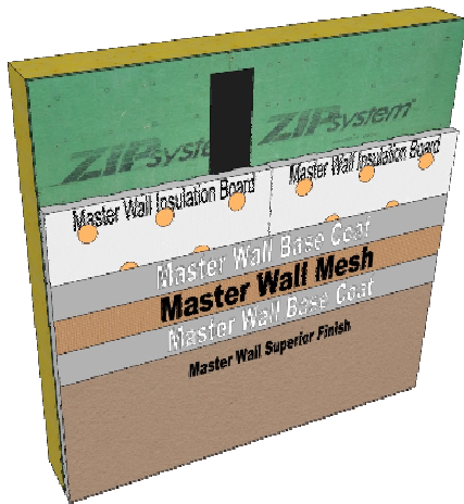
Aggre-flex Drainage EIFS with grooved insulation board
