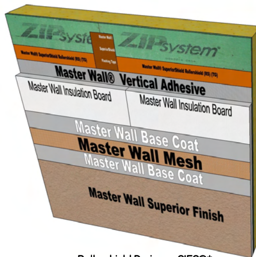
Rollershield Drainage EIFS®* With Rollershield LAB seam treatment
