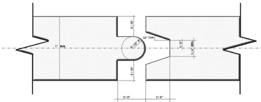
FIGURE 1 – Foam Plastic Tongue and Groove
