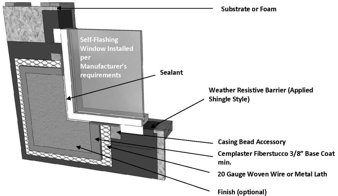
FIGURE 5 – Stucco System at Self-Flashing Window Sill
