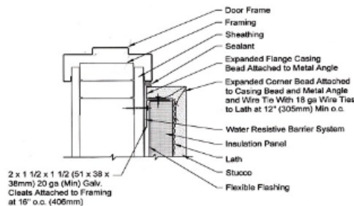
Stucco Door Jamb Detail
