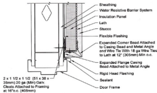
Stucco Door Head Detail
