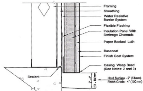
Stucco Base of Wall Detail
