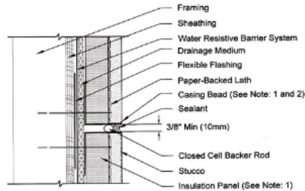
Stucco Horizontal Control Joint
