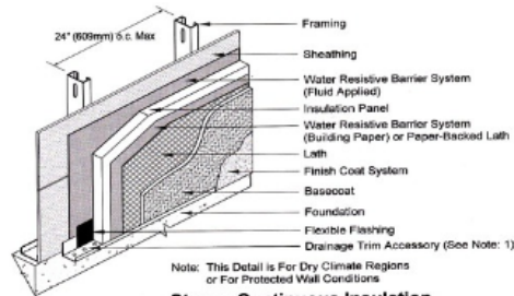
Stucco Continuous Insulation
