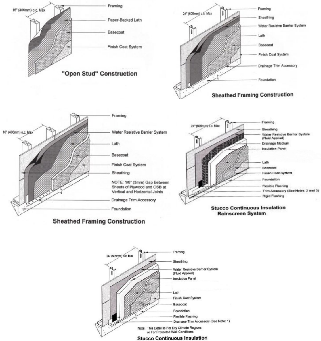
Figure 2 – One Coat FRS Typical Installation Details
