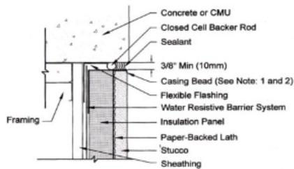
Stucco To Concrete / CMU Joint Detail
