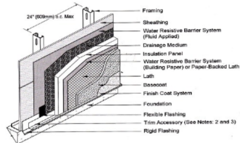
Stucco Continuous Insulation Rainscreen System
