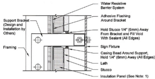
Penetrating Support Bracket Detail
