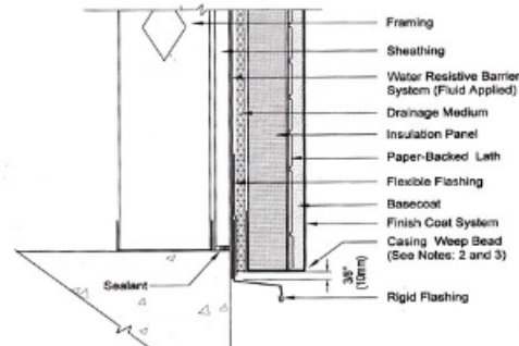
Stucco Base of Wall Detail
