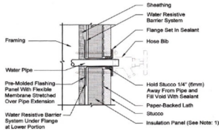
Stucco Hose Bib Through Wall Detail
