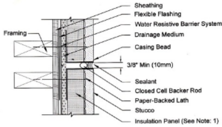
Stucco Vertical Control Joint
