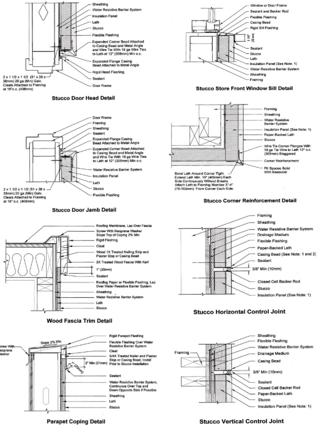
Figure 4 – One Coat FRS Typical Installation Details
