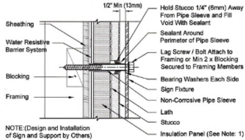
Stucco Through Wall Offset
