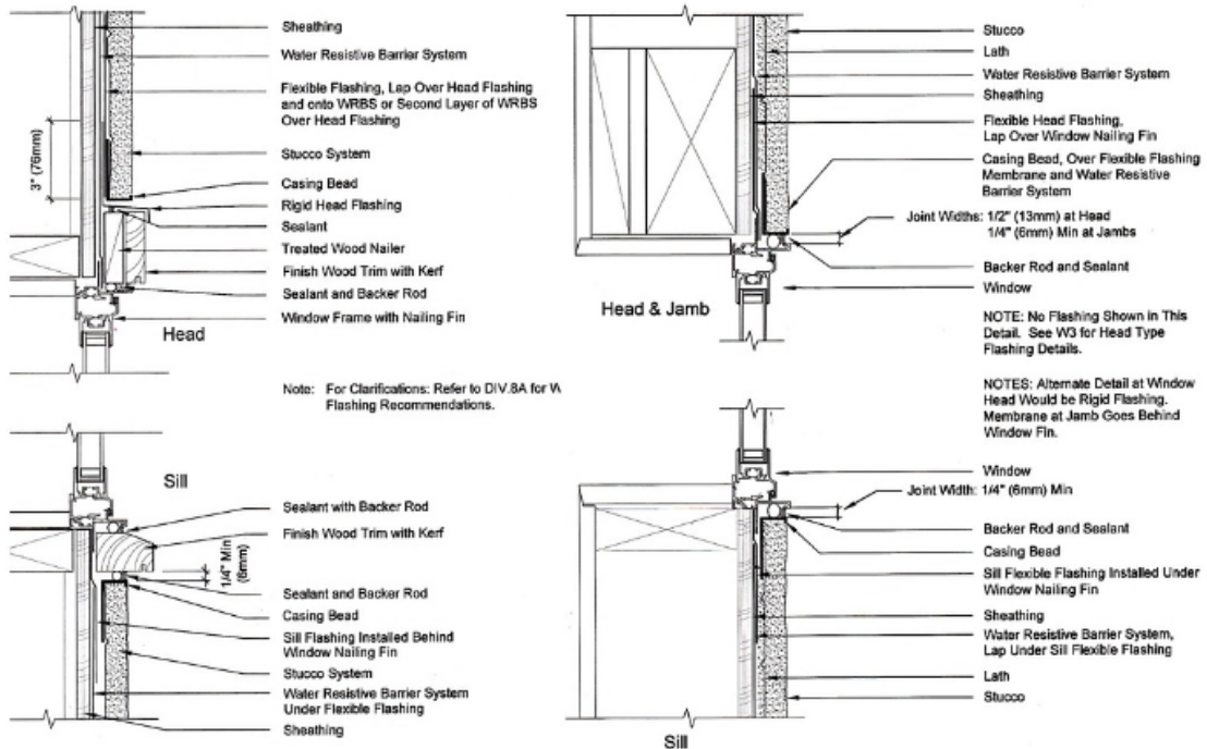
Nail-on Window with Wood Trim
