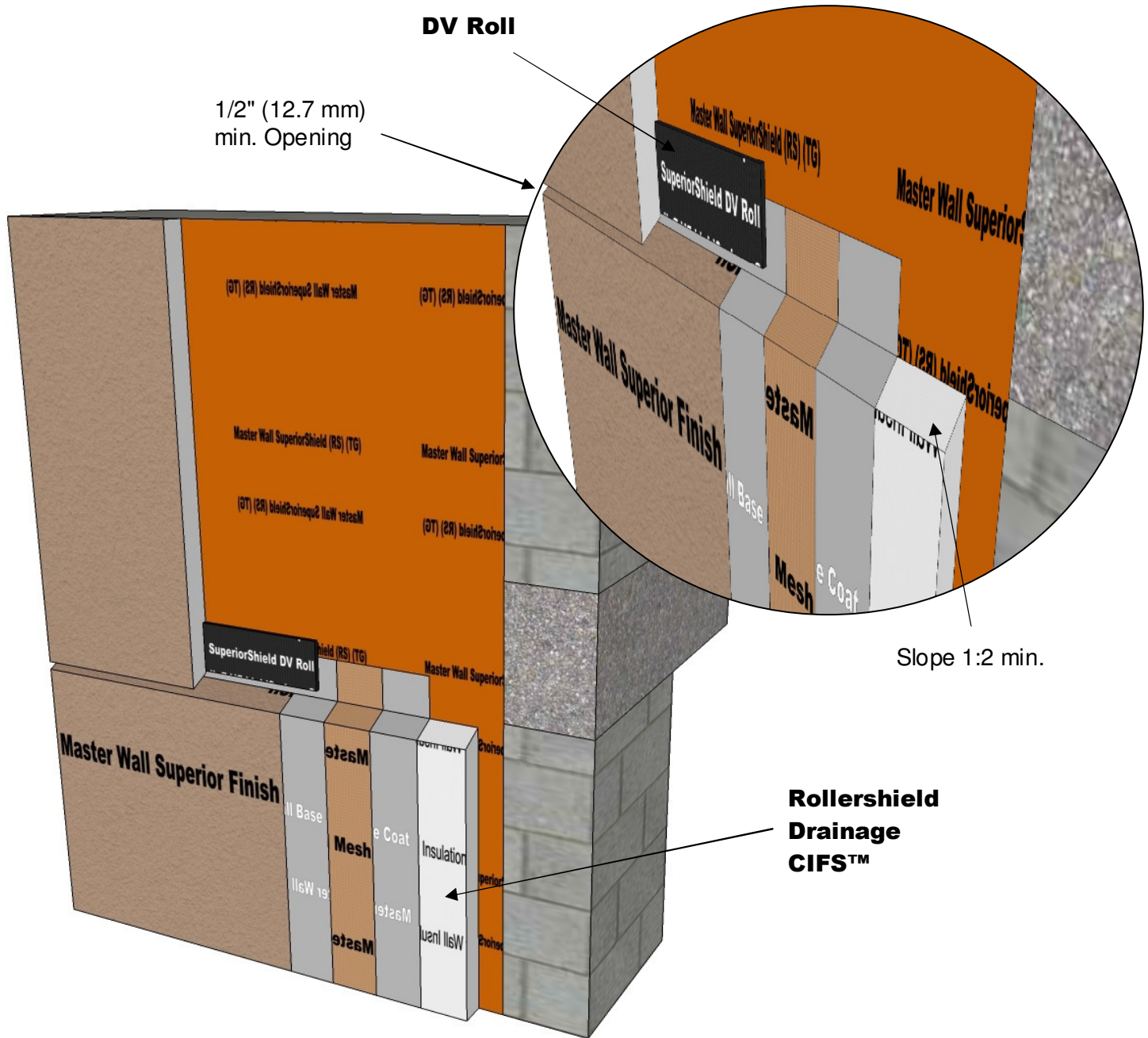
RDCIFS SD 013 FLOOR LINE DRAINAGE DETAIL
