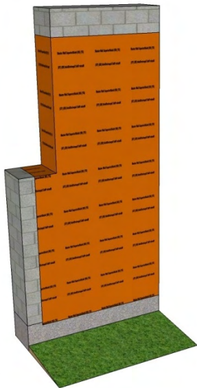
CMU/Masonry Application
